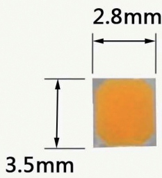
Customized SMD2835(36V) 0.5Watt/chip,120leds/meter.
